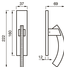
08 CQSW CREMONESE WINDOW HANDLE
