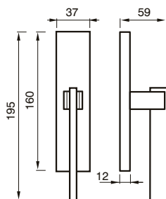
144 CQ CREMONESE WINDOW HANDLE
