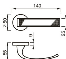
170 RT MANIGLIA C/ROSETTA C/MOLLA HANDLE W/ROSE W/SPRING
