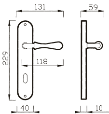
57 PO MANIGLIA C/PLACCA C/MOLLA HANDLE W/PLATE W/SPRING
