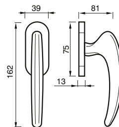
68 DK CREMONESE DK WINDOW HANDLE DK
