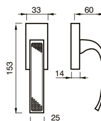
170 DKQ CREMONESE DK WINDOW HANDLE DK
