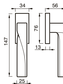
CREMONESE DK WINDOW HANDLE DK
