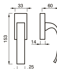
05 DKQ CREMONESE DK WINDOW HANDLE DK
