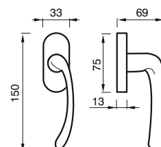
89 DK CREMONESE DK WINDOW HANDLE DK
