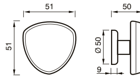
POMOLO C/ROSETTA KNOB W/ROSE
