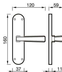
46 C CREMONESE WINDOW HANDLE
