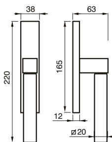
18 C CREMONESE WINDOW HANDLE
