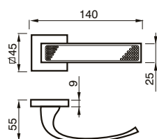
170 RQ MANIGLIA C/ROSETTA C/MOLLA HANDLE W/ROSE W/SPRING
