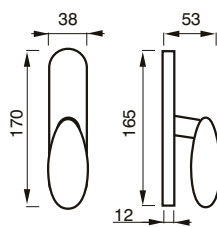
62 C CREMONESE WINDOW HANDLE
