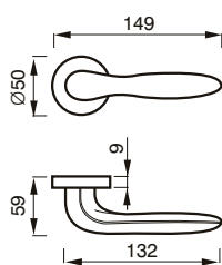
55 R MANIGLIA C/ROSETTA C/MOLLA HANDLE W/ROSE W/SPRING
