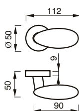
62 PM MANIGLIA C/ROSETTA C/MOLLA HANDLE W/ROSE W/SPRING
