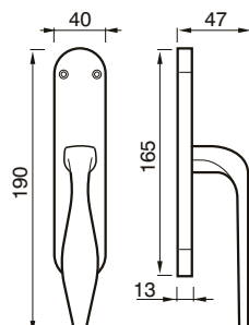
88 C CREMONESE WINDOW HANDLE
