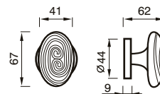
POMOLO C/ROSETTA KNOB W/ROSE
