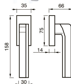
150 DKQ CREMONESE DK WINDOW HANDLE DK
