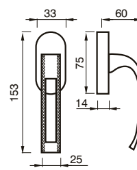
07 DKS CREMONESE DK WINDOW HANDLE DK
