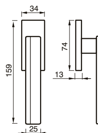
69 DK CREMONESE DK WINDOW HANDLE DK
