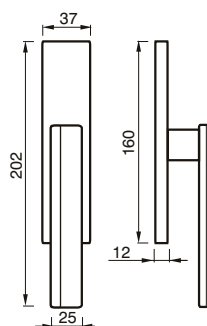
69 C CREMONESE WINDOW HANDLE
