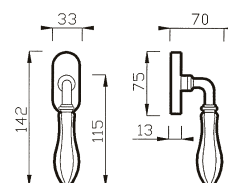
67 DK CREMONESE DK WINDOW HANDLE DK
