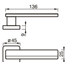
69 R MANIGLIA C/ROSETTA HANDLE W/ROSE
