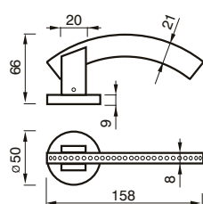
08 RSW MANIGLIA C/ROSETTA C/MOLLA HANDLE W/ROSE W/SPRING
