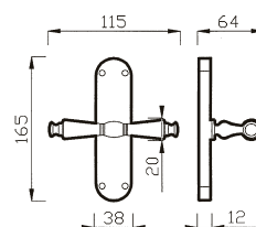
44 C CREMONESE WINDOW HANDLE
