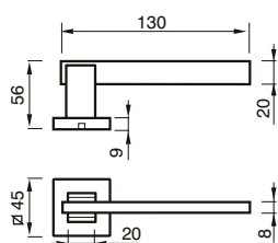
144 RQ MANIGLIA C/ROSETTA C/MOLLA HANDLE W/ROSE W/SPRING
