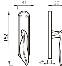
CREMONESE WINDOW HANDLE
