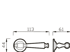
44 RCV MANIGLIA C/ROSETTA C/MOLLA HANDLE W/ROSE W/SPRING
