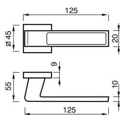
142 RQ MANIGLIA C/ROSETTA C/MOLLA HANDLE W/ROSE W/SPRING
