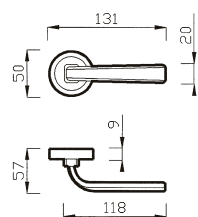
46 R MANIGLIA C/ROSETTA C/MOLLA HANDLE W/ROSE W/SPRING
