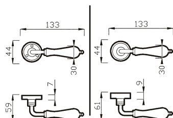
65 RVV - 65 RCV MANIGLIA C/ROSETTA C/MOLLA HANDLE W/ROSE W/SPRING
