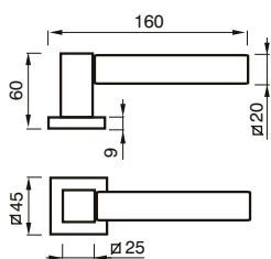
18 R MANIGLIA C/ROSETTA 45 C/MOLLA HANDLE W/ROSE W/SPRING
