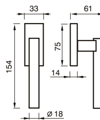
85 DKQ CREMONESE DK WINDOW HANDLE DK
