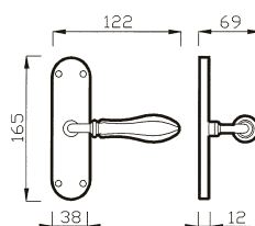
67 C CREMONESE WINDOW HANDLE
