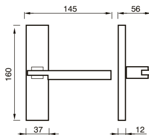
54 C CREMONESE WINDOW HANDLE
