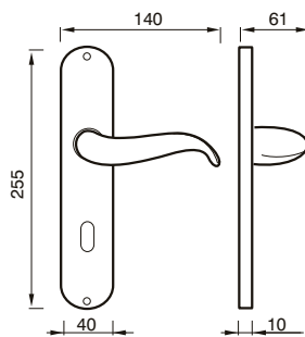
14 P MANIGLIA C/PLACCA HANDLE W/PLATE
