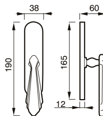
200 C CREMONESE WINDOW HANDLE
