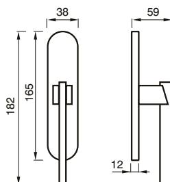
145 C CREMONESE WINDOW HANDLE
