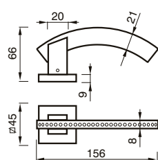
08 RQSW MANIGLIA C/ROSETTA C/MOLLA HANDLE W/ROSE W/SPRING
