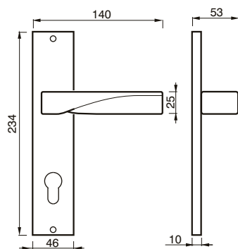
MANIGLIA C/PLACCA C/MOLLA HANDLE W/PLATE W/SPRING
