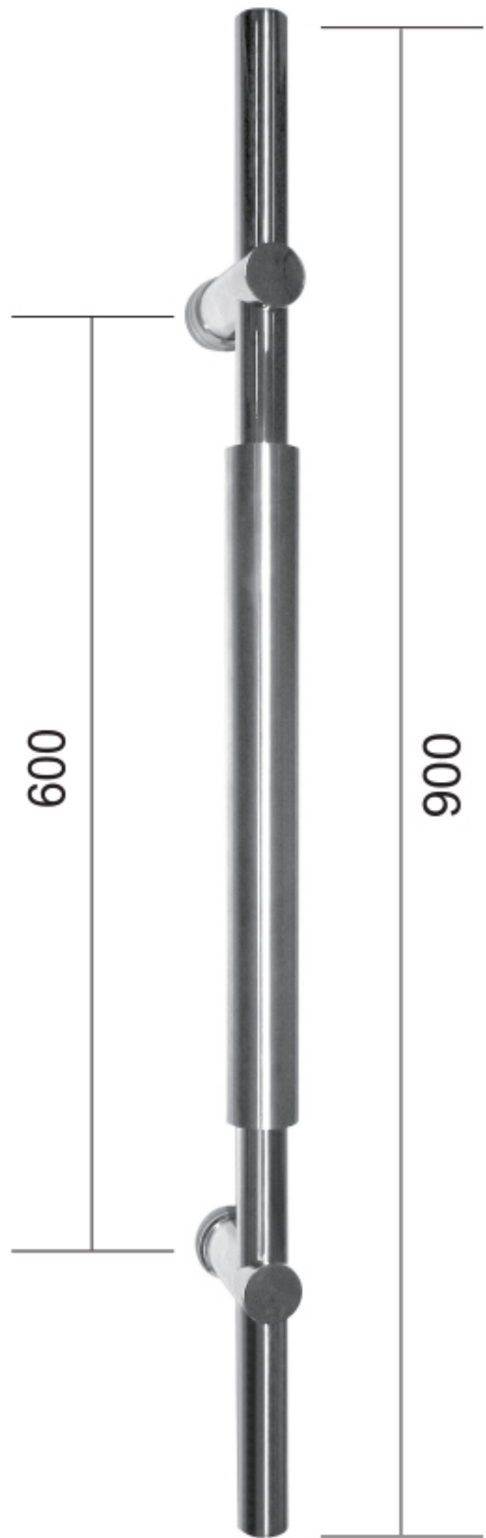
GHD 4502 D32 x 600 x 900mm Material : Stainless Steel Finish : US32D + US32
