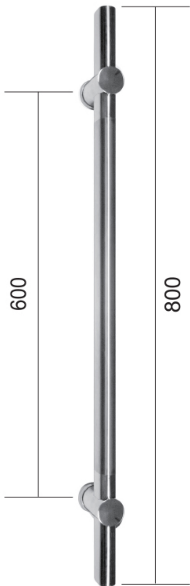
GHD 4503 D25 x 600 x 800mm Material : Stainless Steel Finish : US32D + US32
