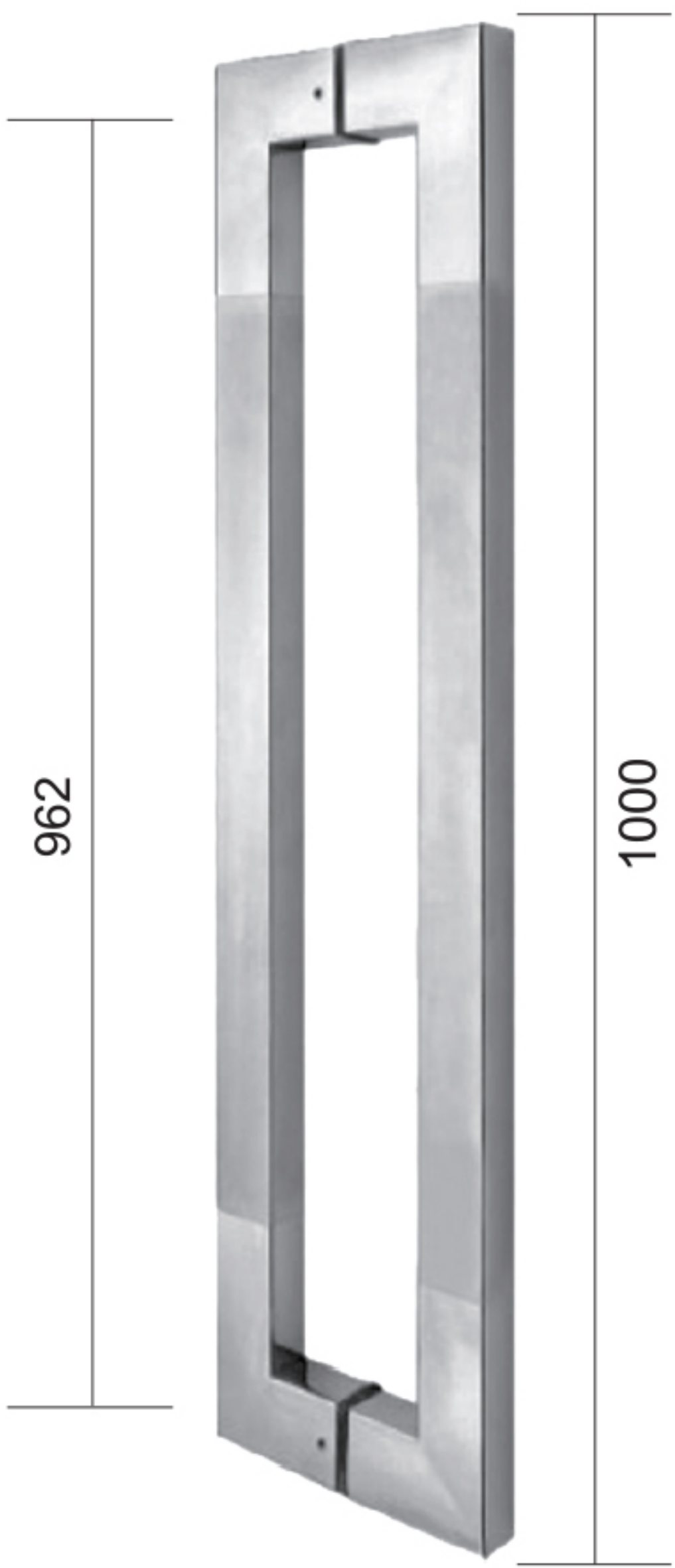
GHD 0036 - D38 x 100cm Material : Stainless Steel Finish : US32 + US32D
