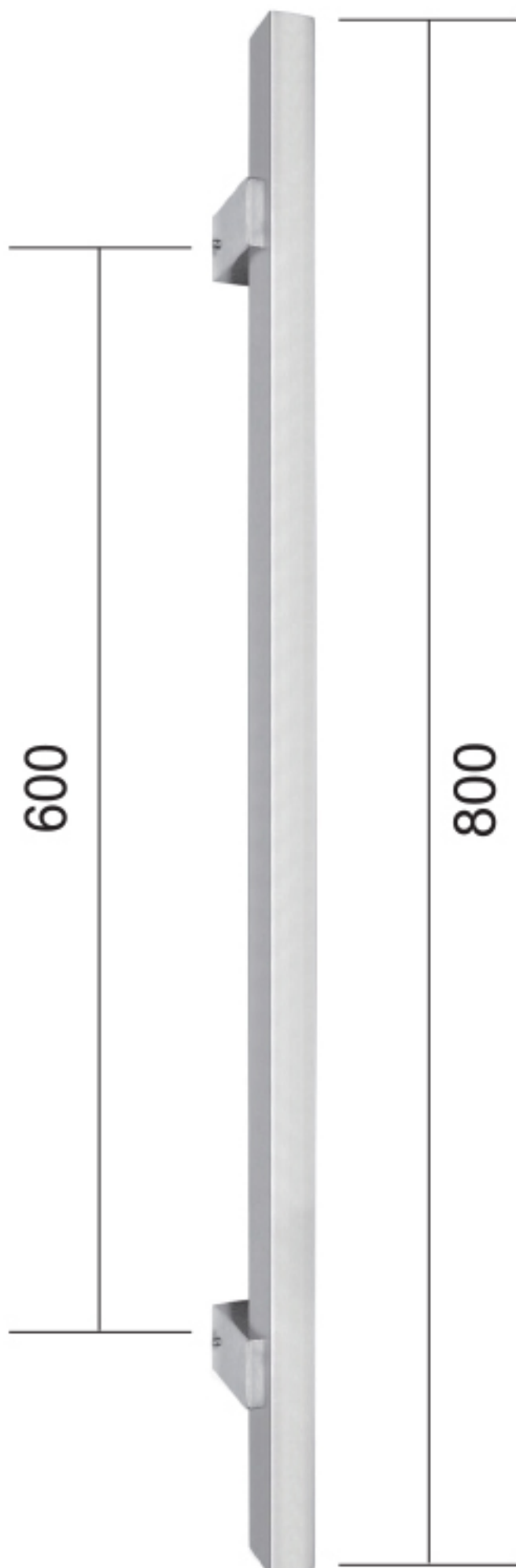
GHD 4504 D38 x 600 x 800mm Material : Stainless Steel Finish : US32D + US32
