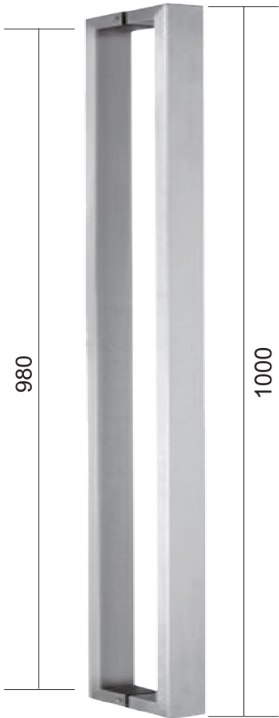
GHD 0037 - D40 x 100cm Material : Stainless Steel Finish : US32D
