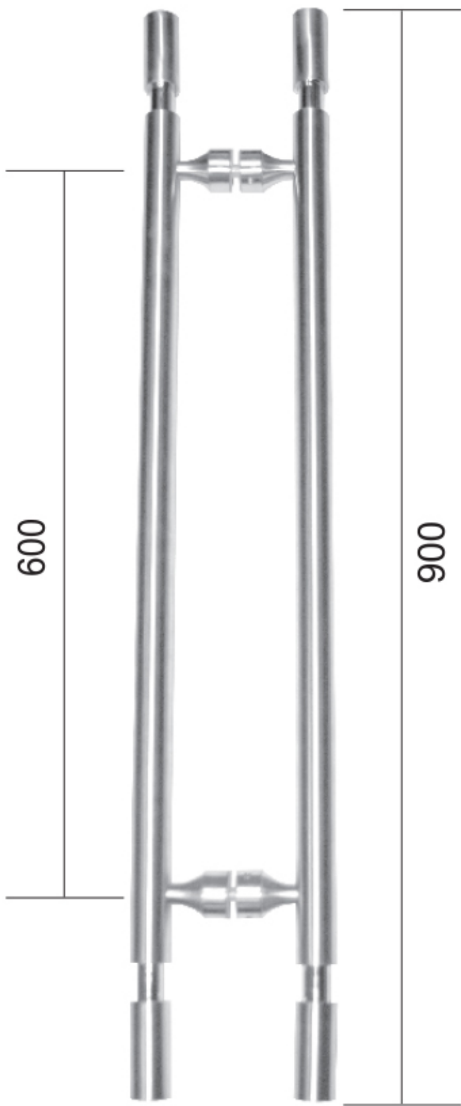
GHD 4501 D32 x 600 x 900mm Material : Stainless Steel Finish : US32D + US32
