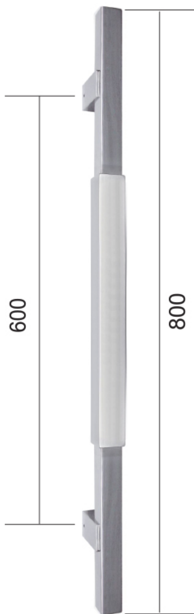
GHD 4505 D30 x 600 x 800mm Material : Stainless Steel Finish : US32D + US32
