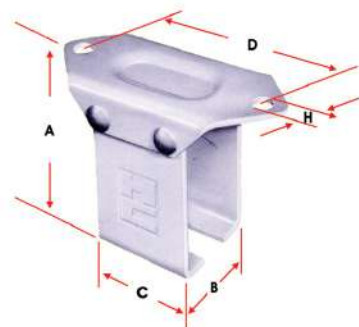
UNIVERSAL SOFFIT FIXING BRACKET
