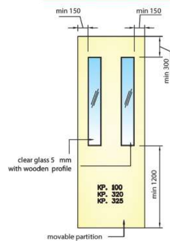
PANEL WITH DOUBLE CLEAR GLASS
